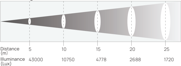
Beam Angle 33.8°
